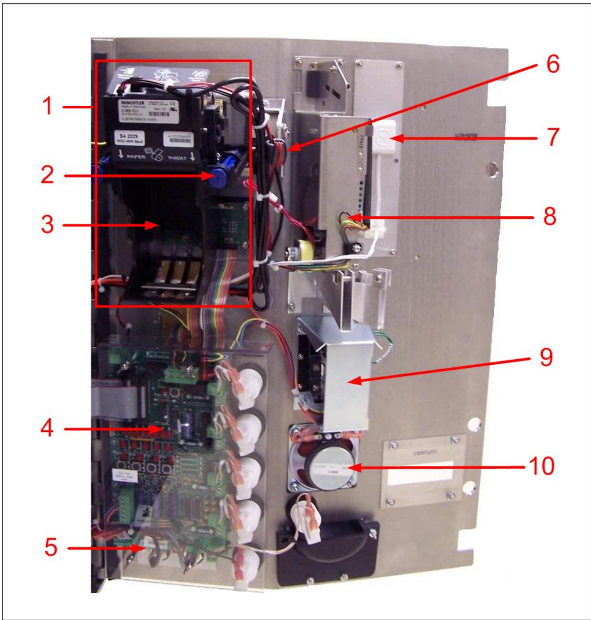
Figure 2. Inside Door
