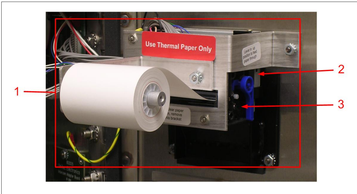
Figure 5. Seiko Printer
